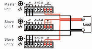
Parallel Connection
